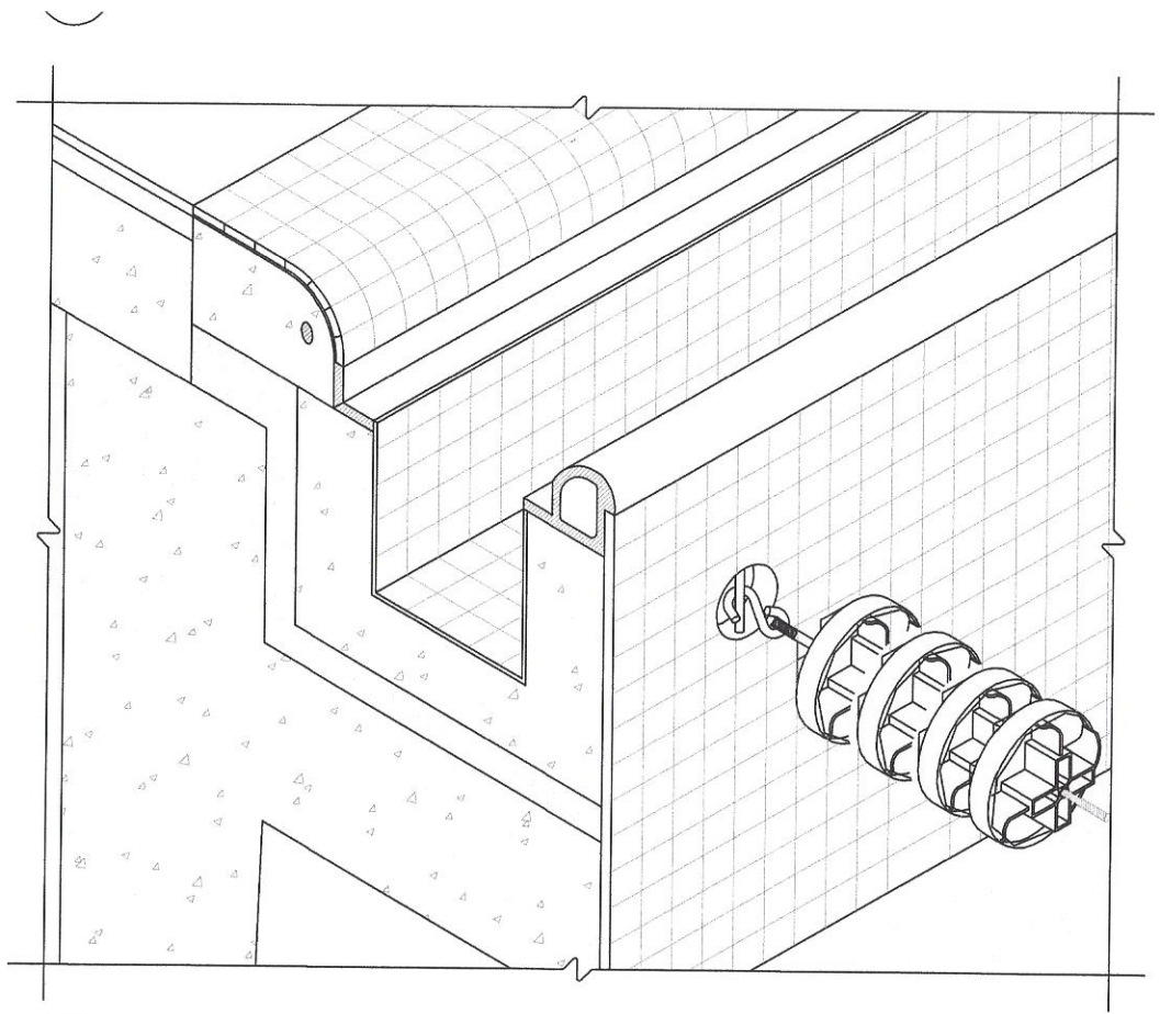
F NATURAL FLOW GUTTER SYSTEM SCALE: 3" = 1'-0"
